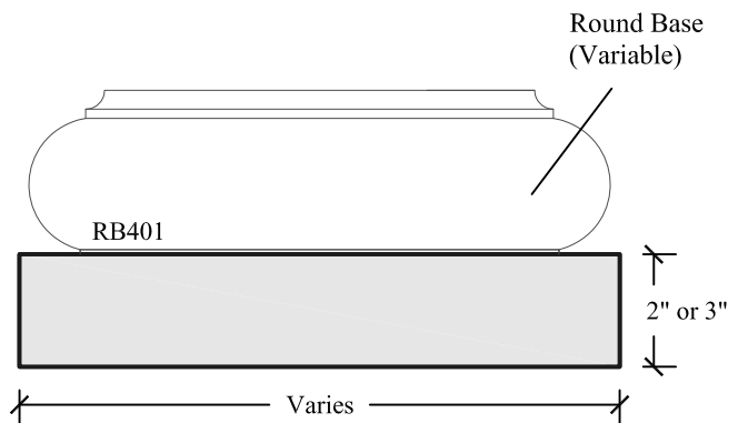
Square Sub-Base
